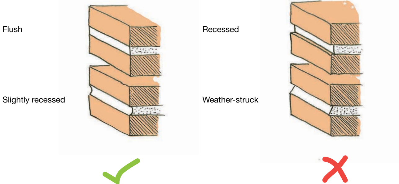
Picture 54. Mortar joint profiles
